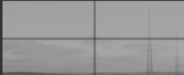
object-fit: none
