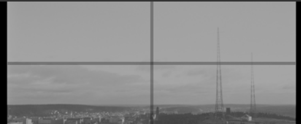
object-fit: cover
